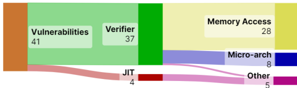
Figure 2: A summary of the types of CVEs reported in each component of eBPF from 2010 to 2023.
